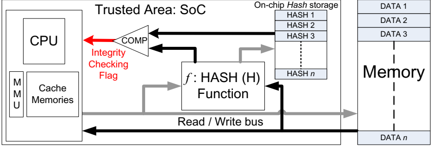
(a) Hash functions: \text{Hash}_n = H(\text{DATA}_n)
