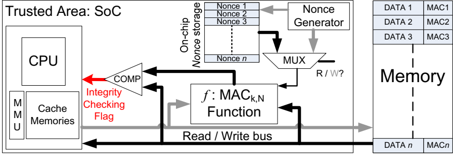
(b) MAC functions: \text{MAC}_n = \text{MAC}_k(\text{DATA}_n)
