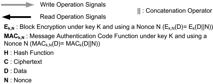
(c) Block-Level AREA: C_n = E_k(D_n || N_n)
