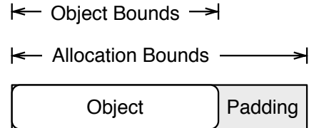
Figure 1: Allocated memory is often padded to a particular alignment boundary, and hence can be larger than the requested object size. By checking allocation bounds rather than object bounds , we allow benign accesses to the padding, but can significantly reduce the cost of bounds lookups at runtime.
