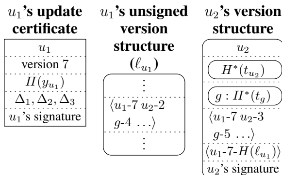
Figure 7: A pending update by user u_1 , reflected in user u_2 's version structure.
